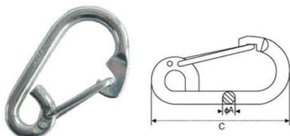
Spring Hook 圆弧简易弹簧钩
