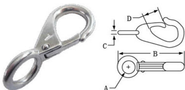
Egg Shaped snap Hook 蛋型弹簧钩
